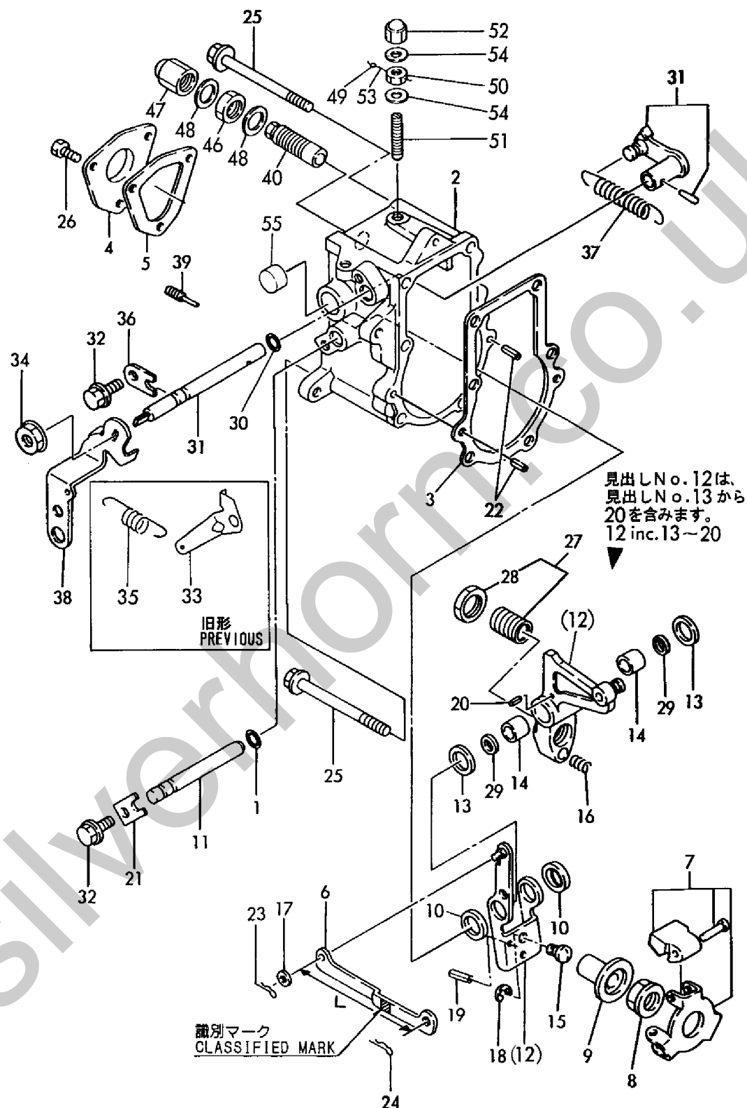
Fig. 13 ガバナ GOVERNOR
